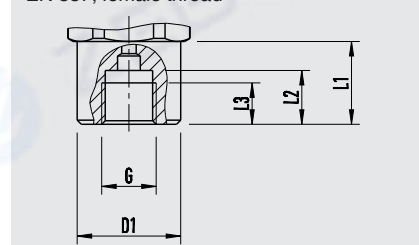
EN 837, female thread
