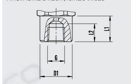
ANSI/ASME B1.20.1, female thread
